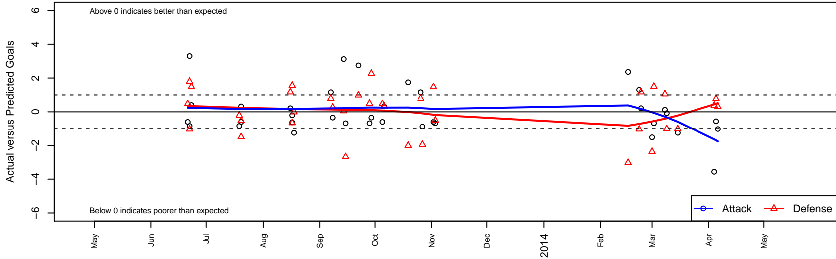
FC Salmon Creek Nemesis Yellow G02 Dots are actual minus expected GF (blue circles) and GA (red triangles). Blue line is smoothed change in attack strength. Red is smoothed change in defense strength.
